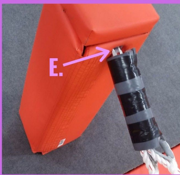
A. Fidget Ladder B. Pit (Air Bag Pictured) C. Anchor Posts D. Perimeter Padding E. Connection Hardware (Ladder to Post)
